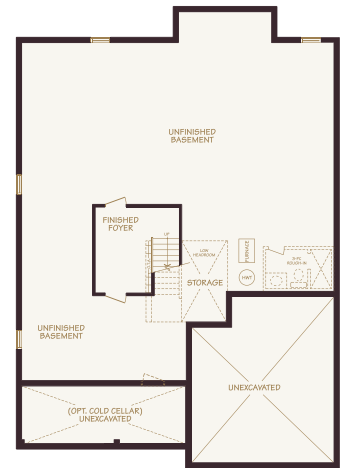
basement plan
