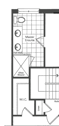
Partial Optional Master Ensuite Elevation A & B
