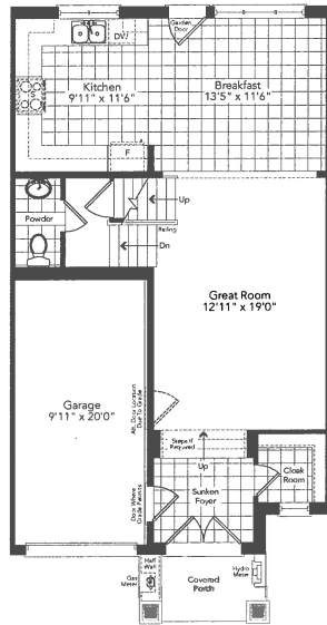
Optional Ground Floor Elevation A
