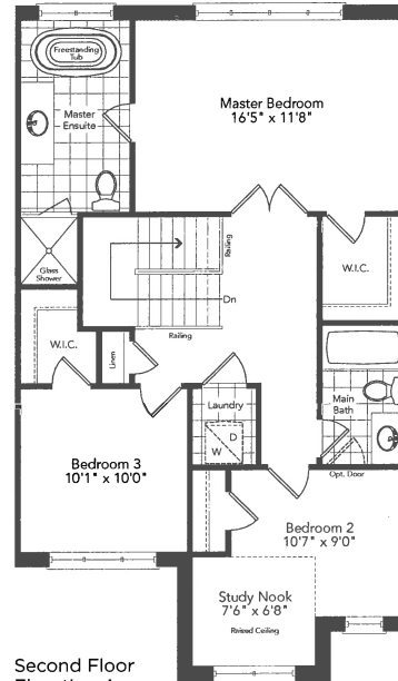
Second Floor Elevation A
