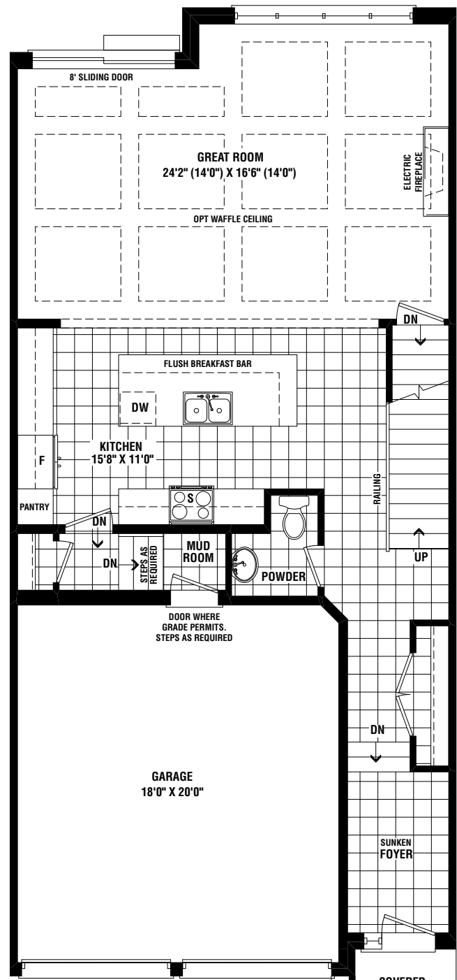
GROUND FLOOR ELEV. 'B-2'
