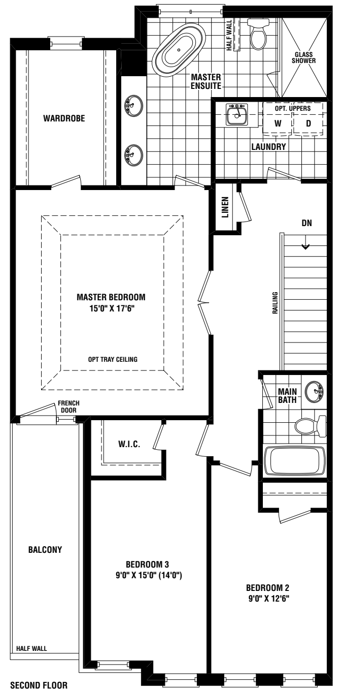
SECOND FLOOR ELEV. 'B-2'
